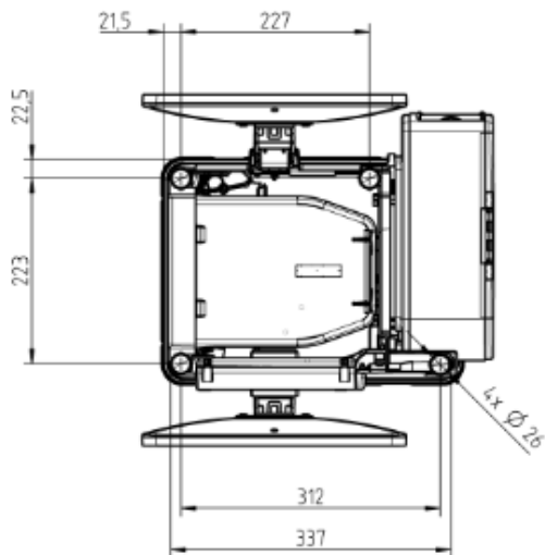
Q1_expert_100_top_view_01
